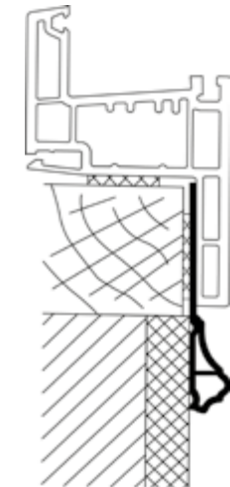
MR9015 en application
